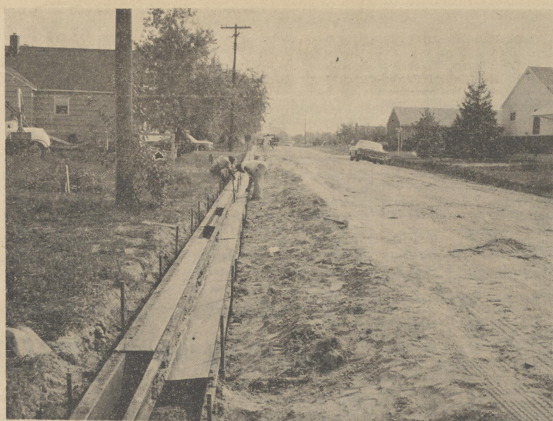
THESE FORMS WILL MAKE CURVES—Workmen are shown laying forms for a one-piece gutter and curb on the eastern side of Dixon Street between Shaw and Smith Avenues in Harrington Manor.
