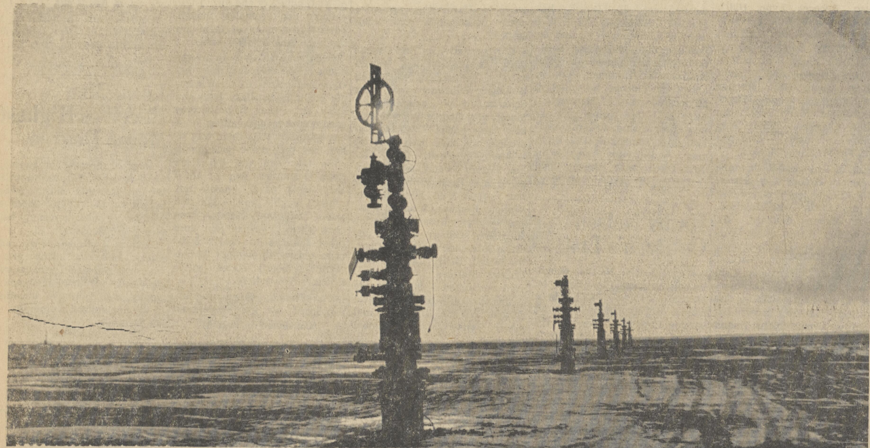
This "Christmas Tree" is black and stands in rigid solitude on the North Slope of Alaska. The device, nicknamed for its unusual shape, is a special assembly of valves and gauges which cap a waiting Alaskan oil well. When approved, the proposed trans Alaska oil pipeline will move the oil from the Prudhoe Bay fields to the ice-free port of Valdez, where it will move by tankers to the West Coast.
