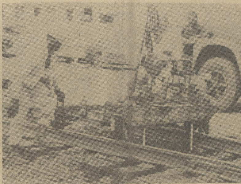
inserted each tie in the right spot. The machine in the center photo raised each rail as vibrations forced crushed stone under it. Then another was used to lift the rail so that men [right photo] could slip grooved metal plates between tie and
