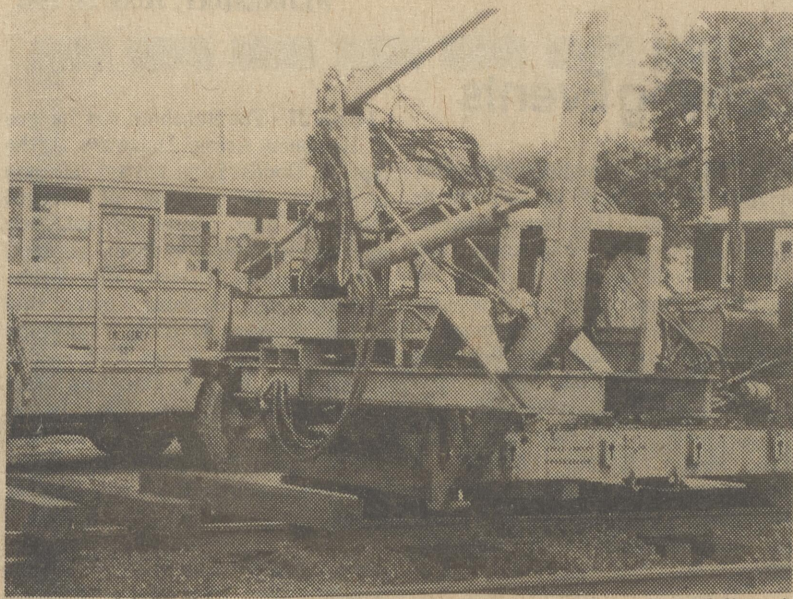
A LINE UP OF MEN AND MACHINES went to work on Conrail lines in Harrington last week as several hundred ties were replaced. The machines can do in days what used to take months. After spaces were tunneled out and ties laid across the track at precise intervals, another mechanical marvel [left picture]
